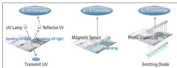
<Ultraviolet Sensor>
